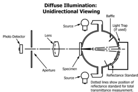
FIG. 2 Spectrophotometer With Diffuse Illumination
