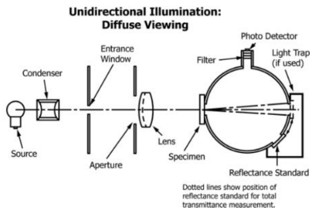
FIG. 1 Schematic of Hazemeter
